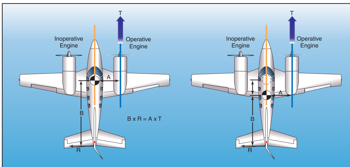
Figure 12-20. Effect of CG location on yaw.
