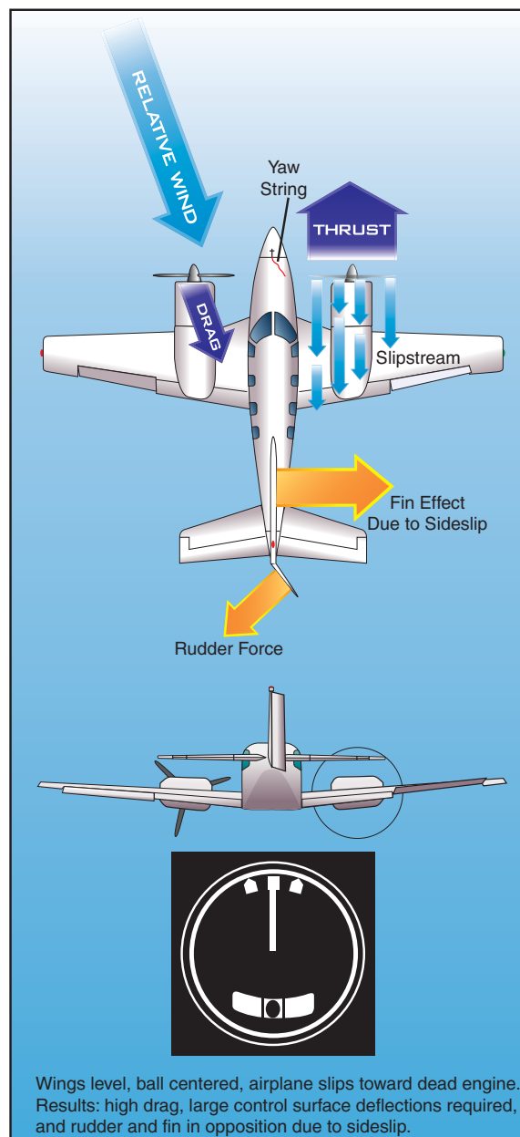
Figure 12-16. Wings level engine-out flight.
