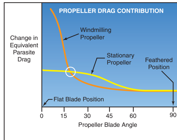
Figure 12-3. Propeller drag contribution.
