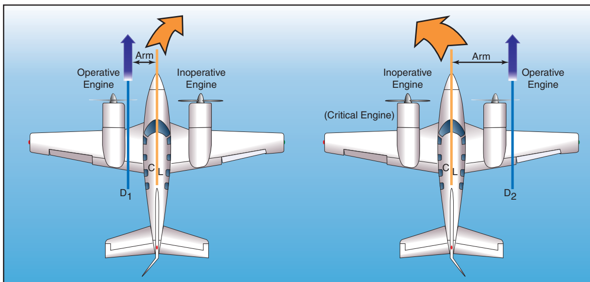
Figure 12-19. Forces created during single-engine operation.
