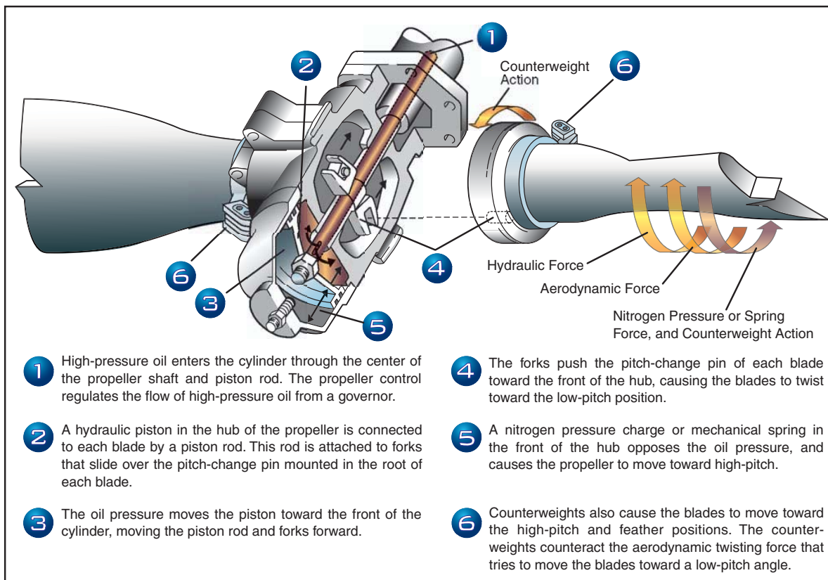
Figure 12-4. Pitch change forces.
