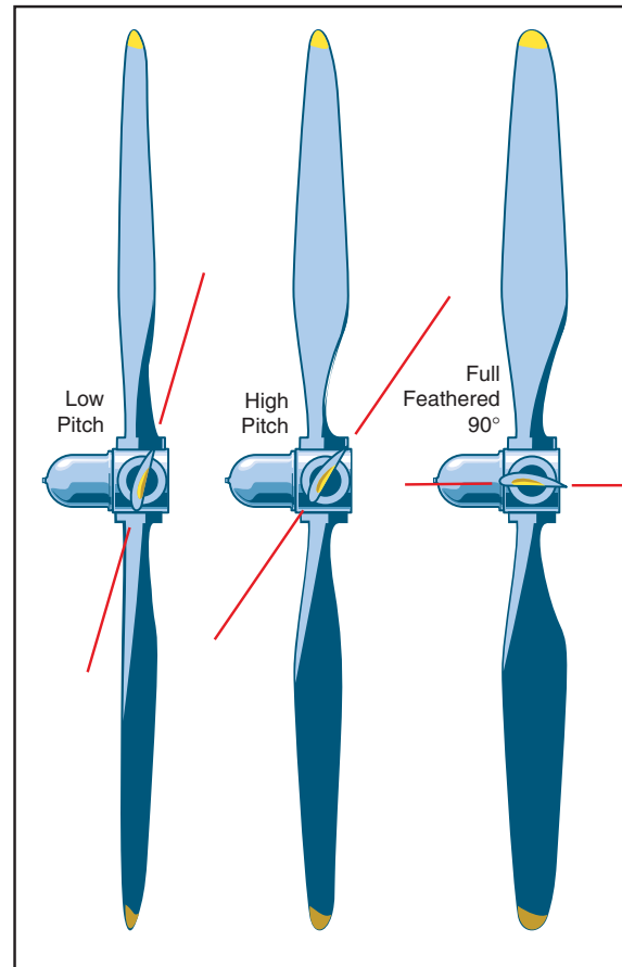
Figure 12-2. Feathered propeller.
