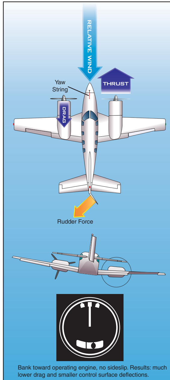
Figure 12-18. Zero sideslip engine-out flight.
