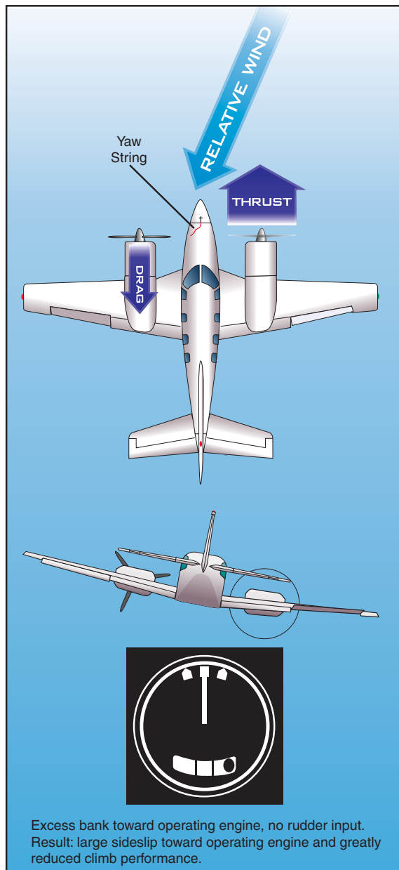
Figure 12-17. Excessive bank engine-out flight.
